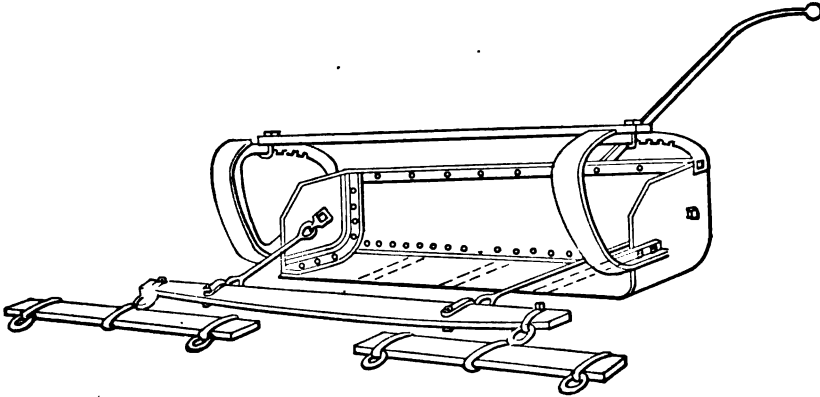
FIG. 29.—Fresno Scraper.
